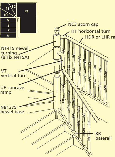
Fig 3D Top landing 180° turn with winders
