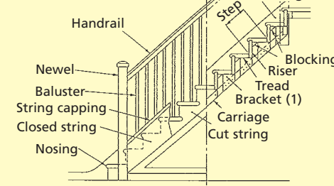
Fig 1 Elevation and section
