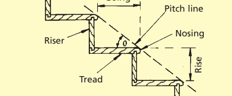
Fig 3 Balustrades and handrails
