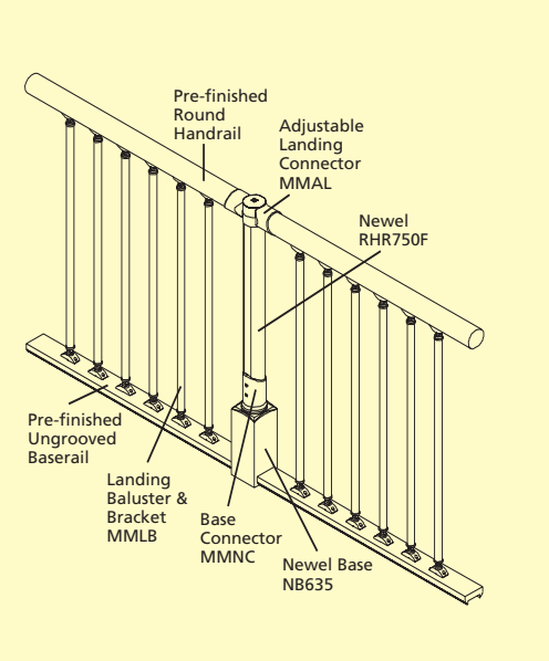
Fig 3F Continuous rail over newel
