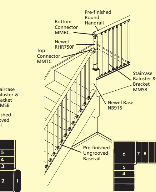
Fig 2A Quarter turn with landing
