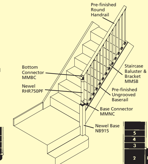
Fig 1C Dogleg with bullnose step
