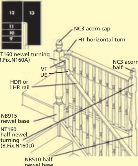
Fig 3B Top landing with 180° turn
