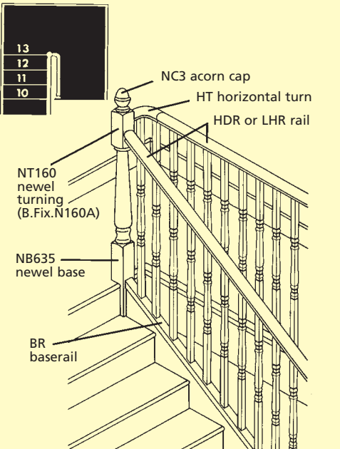
Fig 3C Top landing with 180° turn
