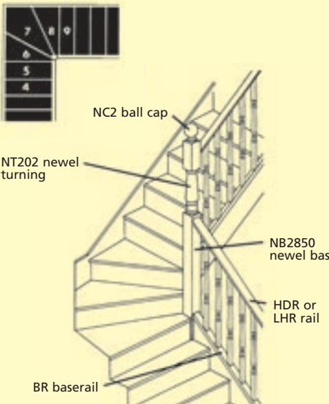
Fig 2D Quarter turn with three winders
