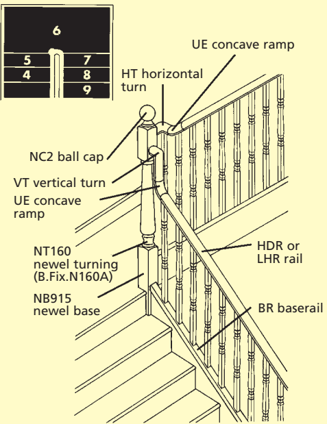
Fig 2H Half turn with extended landing
