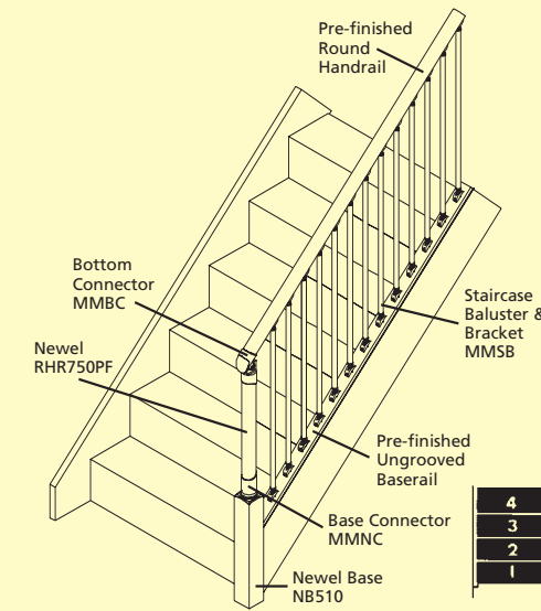
Fig 1A Straight with straight step
