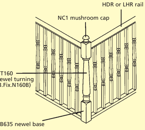
Fig 3F 90° turn with straight rail (with newel)
