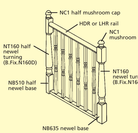
Fig 3H Top landing with 90° turn - Continuous Handrail System
