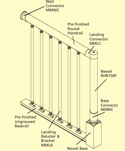
Fig 3G Landing or horizontal balustrading only
