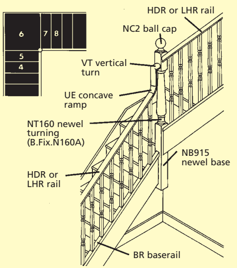
Fig 2A Quarter turn with landing
