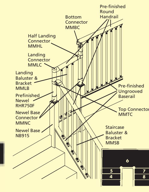
Fig 2C Half turn with extended landing
