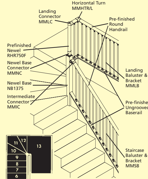
Fig 3D Top landing, 180° turn with winders
