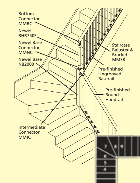
Fig 2B Quarter turn with three winders
