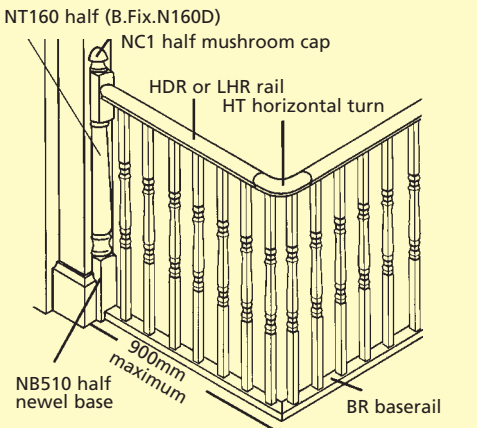
Fig 3E 90° turn with straight rail (without newel)
