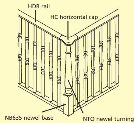
Fig 3L 90° Turn with continuous rail (with newel)
