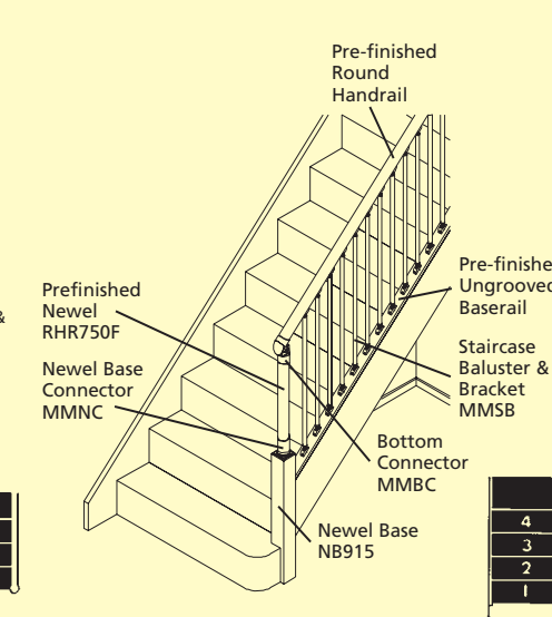
Fig 1B Straight with bullnose step
