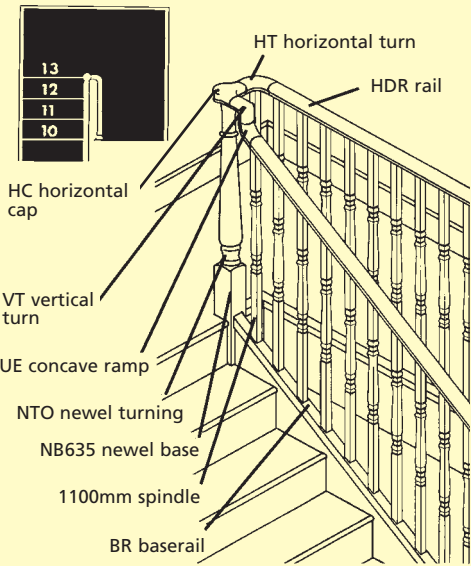
Fig 3L 90° Turn with continuous rail (with newel)
