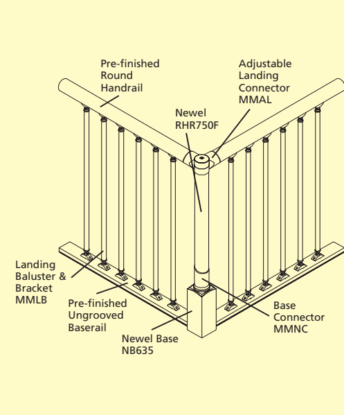
Fig 3E 90° turn with straight rail (with newels)
