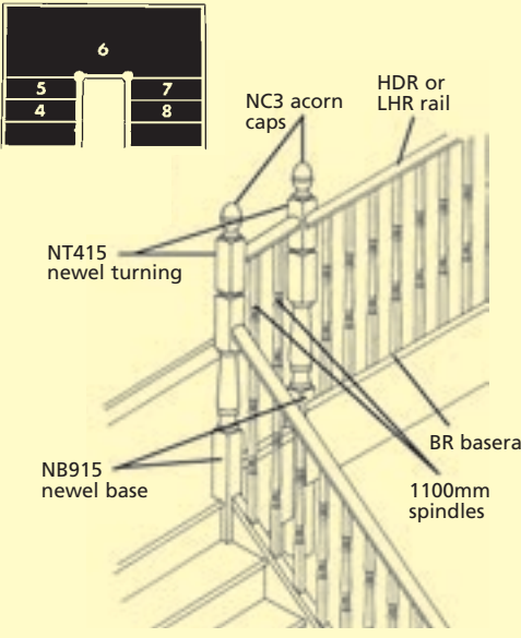
Fig 2H Half turn with extended landing
