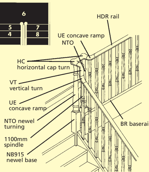
Fig 2K Half turn with landing - Continuous Handrail System minimum distance between centres of strings 150mm
