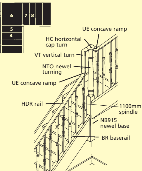
Fig 2J Quarter turn with landing - Continuous Handrail System
