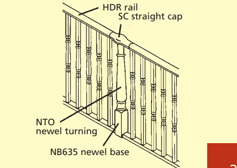
Fig 3J Continuous rail over newel
