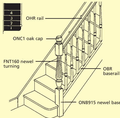
Fig 4B Quarter turn with landing - Classic Oak
