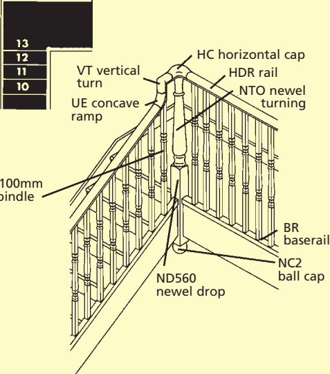
Fig 3J Continuous rail over newel
