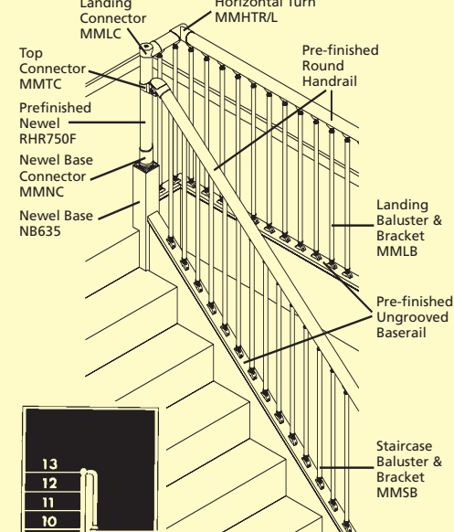
Fig 3C Top landing with 180° turn
