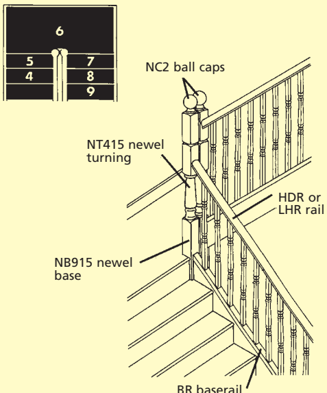
Fig 2F Half turn with landing - minimum distance between centres of strings 82/90mm, 2 newel bases side by side 82 or 90mm section
