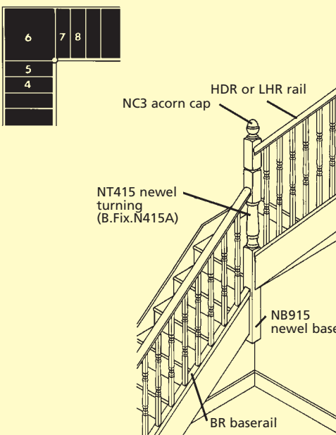
Fig 2C Quarter turn with three winders
