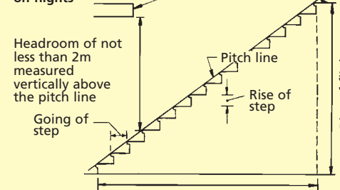
Fig 4 Restrictions on flights
