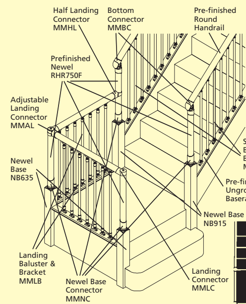
Fig 1E Dogleg with double bullnose and pulpit end
