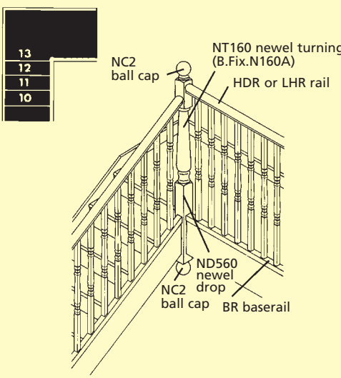
Fig 3B Top landing with 180° turn
